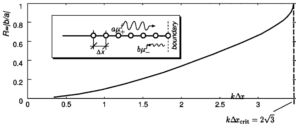
FIG. 12. Discrete coefficient of reflection for the 1D Helmholtz equation.
